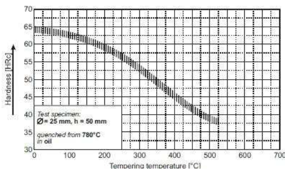
Tempering Diagram
